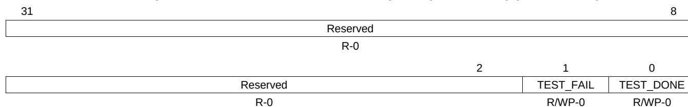
Figure 7-8. Self-Test Global Status Register (STCGSTAT) (offset = 14h)
