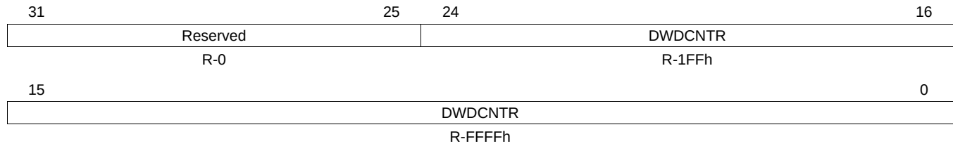
Figure 12-36. RTI Watchdog Down Counter Register (RTIDWDCNTR) [offset = A0h]
