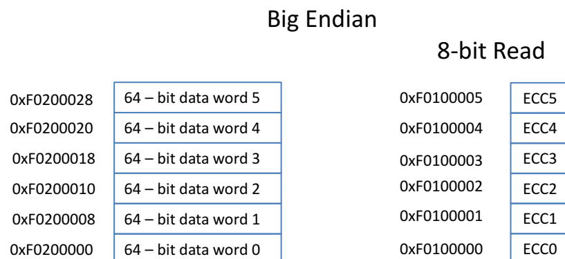
Figure 4-2. ECC Organization for Bank 7 (72-Bits Wide)
