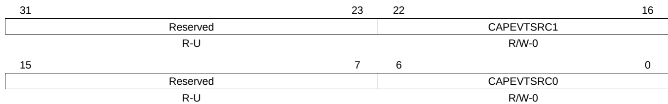
Figure 14-37. Capture Event Register (CAPEVT) [offset = 78h]
