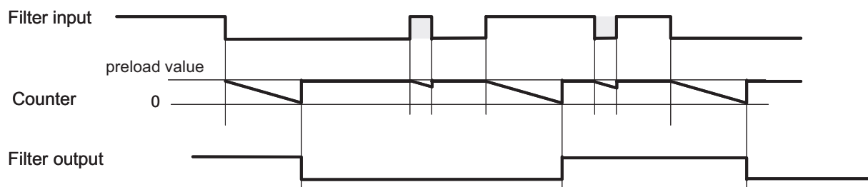
Figure 17-26. Suppression Filter Counter Operation
