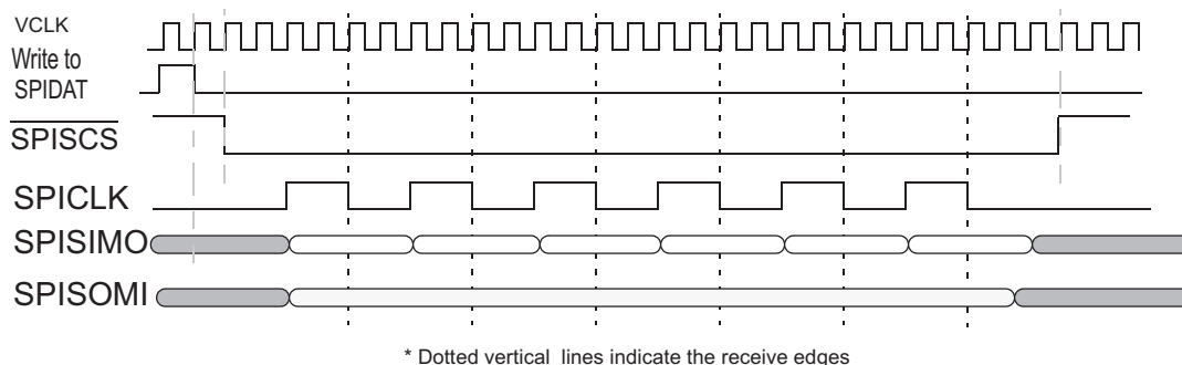
Figure 21-68. SPI/MibSPI Pins During Master Mode 4-pin with \overline{\text{SPISCS}} Configuration
