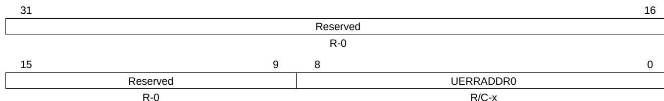
Figure 21-57. TXRAM Uncorrectable Parity Error Address Register (UERRADDR0) [offset = 12Ch]
