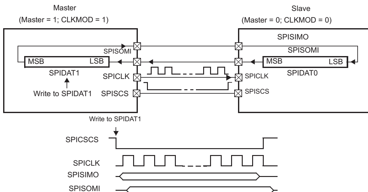
Figure 21-3. Operation with \overline{\text{SPISCS}}
