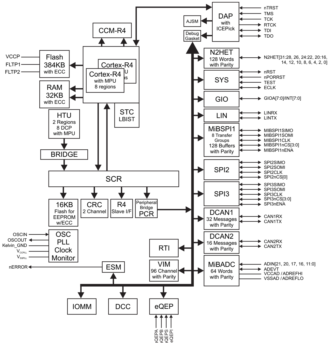
Figure 1-1. Block Diagram
