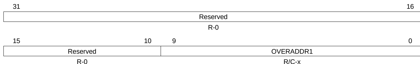
Figure 21-56. RXRAM Uncorrectable Parity Error Address Register (UERRADDR1) [offset = 128h]
