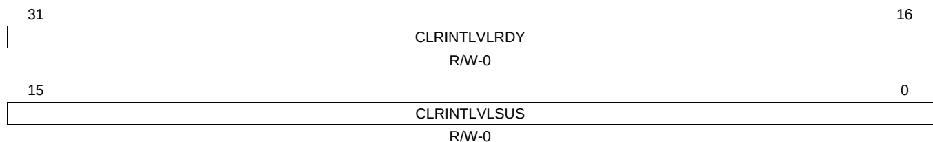
Figure 21-48. Transfer Group Interrupt Level Clear Register (TGITLVCR) [offset = 80h]
