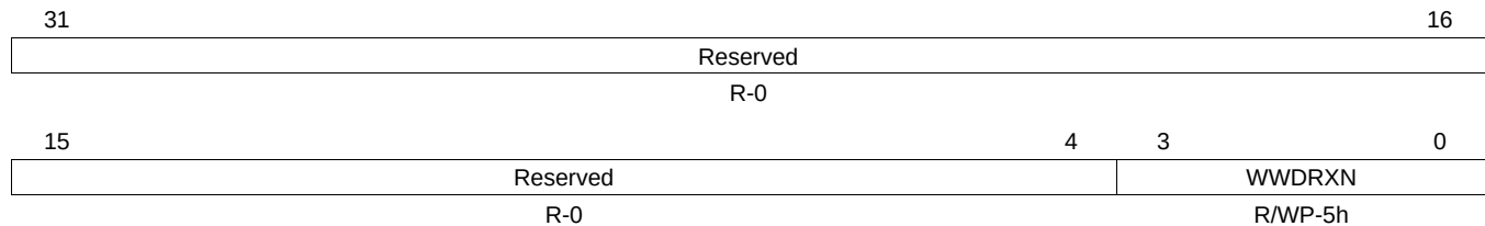
Figure 12-37. Digital Windowed Watchdog Reaction Control (RTIWWDRXNCTRL) [offset = A4h]
