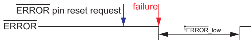
Figure 11-8. \overline{\text{ERROR}} Pin Timing - Example 5
