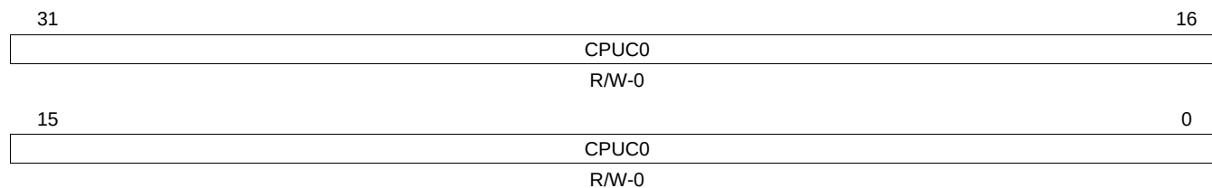
Figure 12-13. RTI Compare Up Counter 0 Register (RTICPUC0) [offset = 18h]
