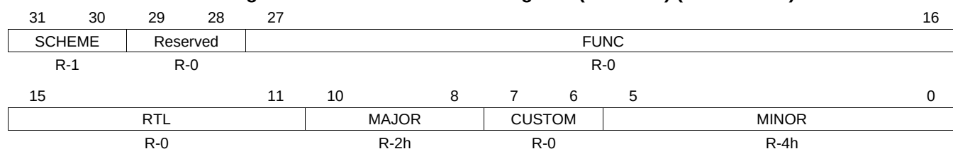
Figure 10-8. DCC Revision ID Register (DCCREV) (offset = 04h)
