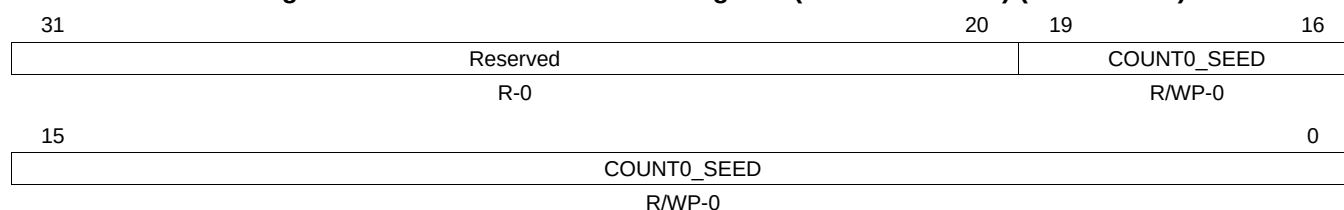
Figure 10-9. DCC Counter0 Seed Register (DCCCNT0SEED) (offset = 08h)
