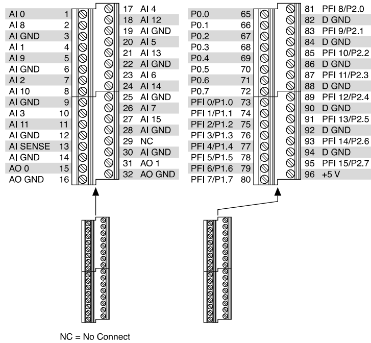
Figure 9. NI USB-6221 Screw Terminal Pinout
