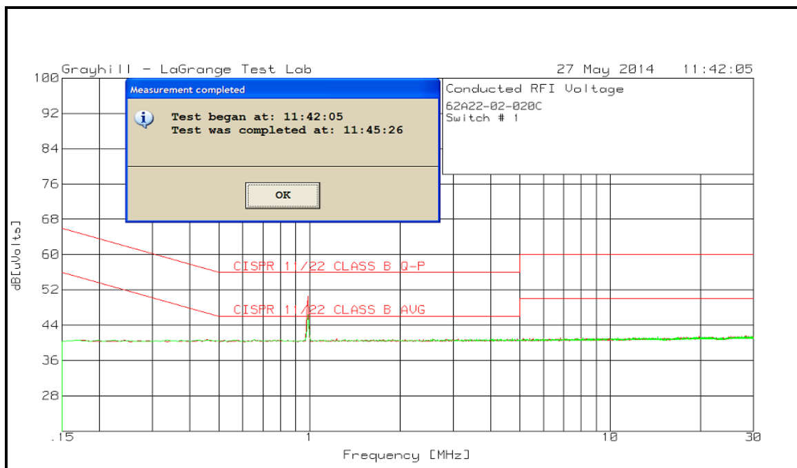
Figure 8 – Conducted Emissions Results
