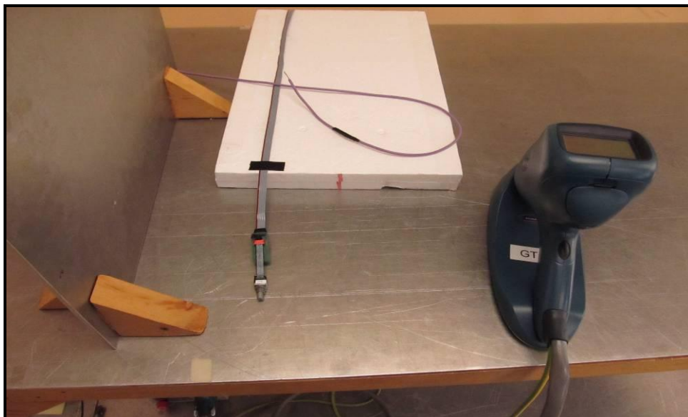
Figure 9 – Electrostatic Discharge Test Setup (Powered)
