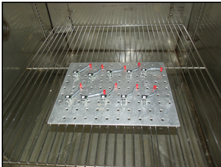
Figure 12 – High Storage Test Setup
