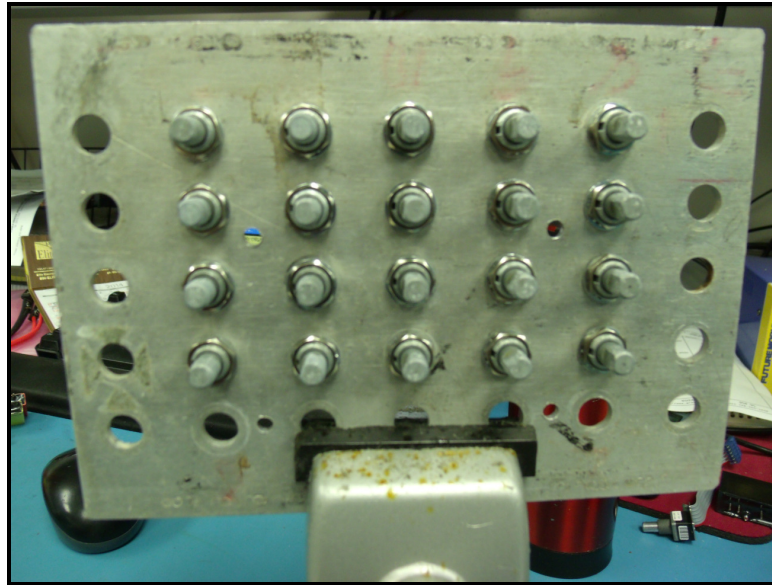
Figure 1– Torque Setup
