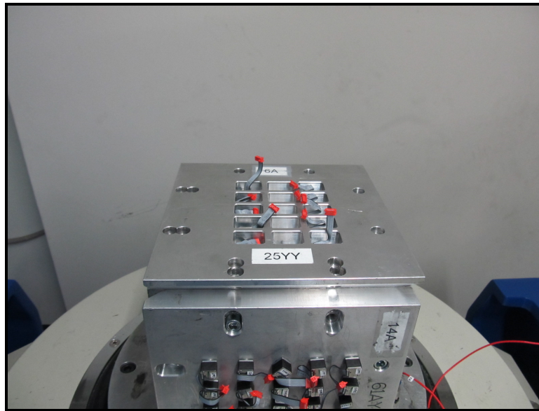
Figure 15 – Random Vibration Test Setup
