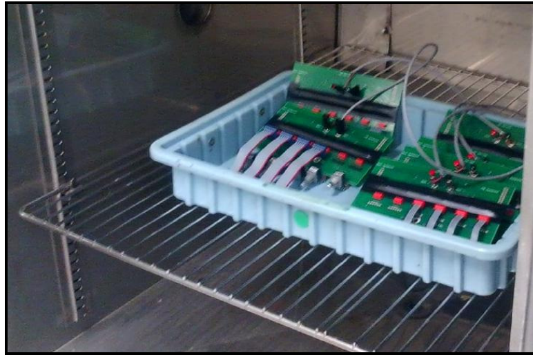
Figure 10 – Operating High Temperature Test Setup
