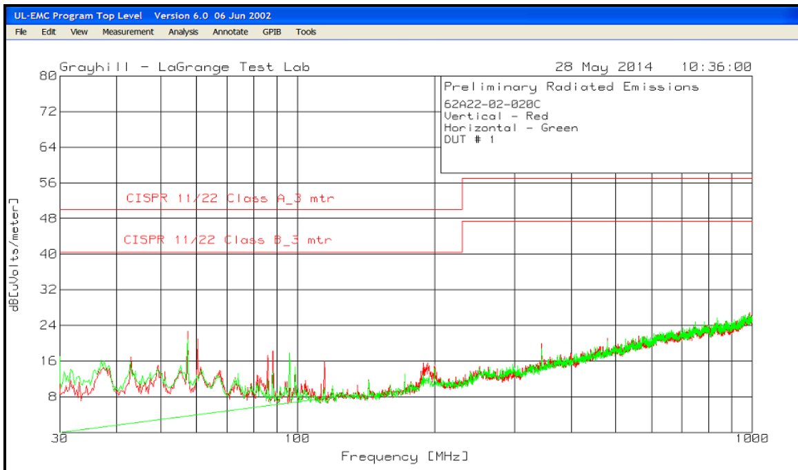
Figure 5 – Radiated Emissions Results (Red Vertical, Green Horizontal)
