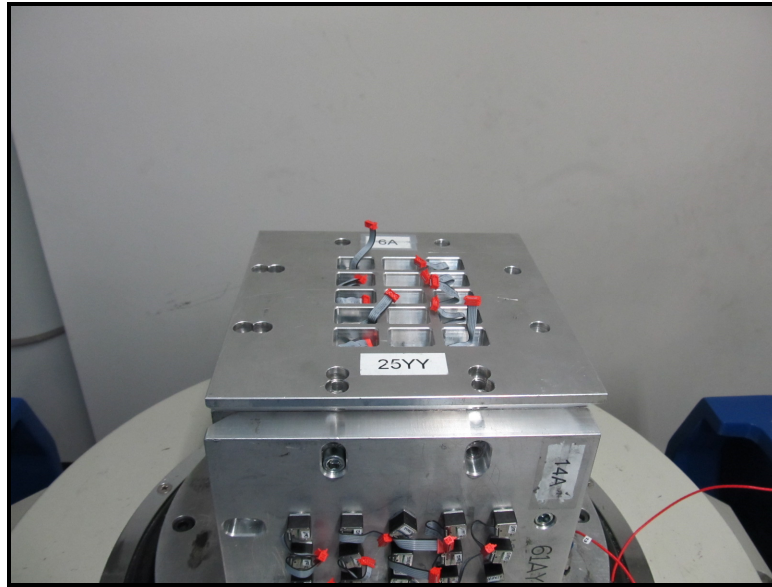
Figure 17 – Mechanical Shock Test Setup
