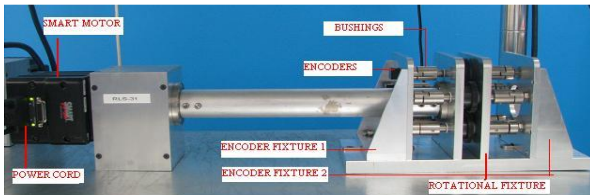
Figure 1 – Rotational Life Setup
