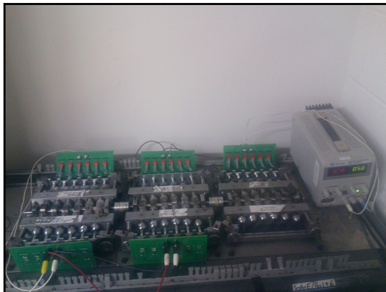
Figure 13 – Push Button Life Test Setup
