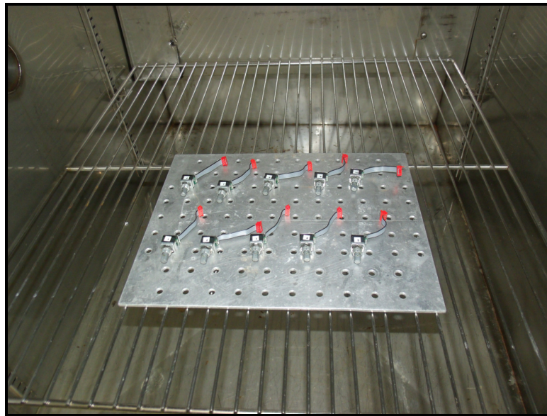
Figure 1 – Storage Low Temperature Test Setup
