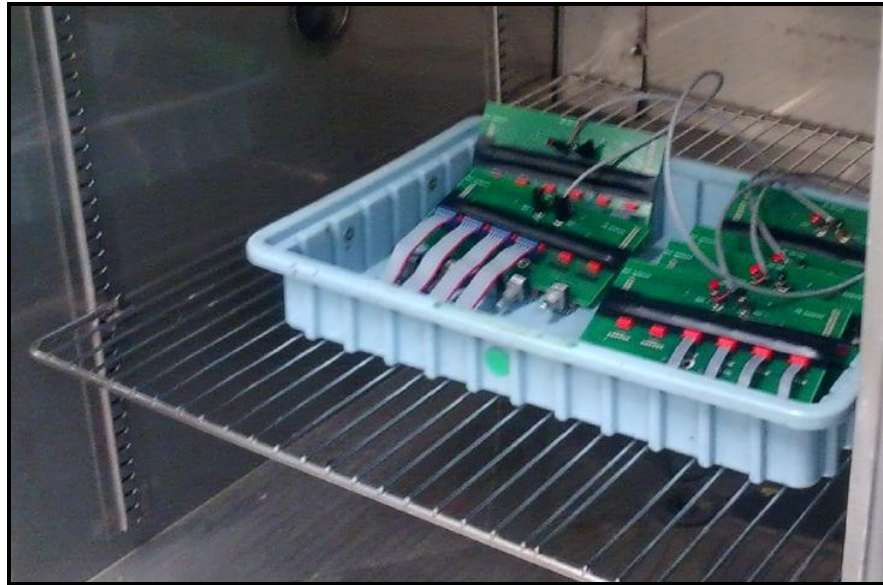
Figure 11 – Operating Low Temperature Test Setup
