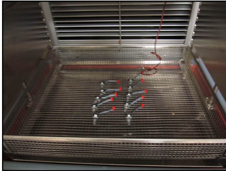
Figure 14 – Thermal Shock Test Setup
