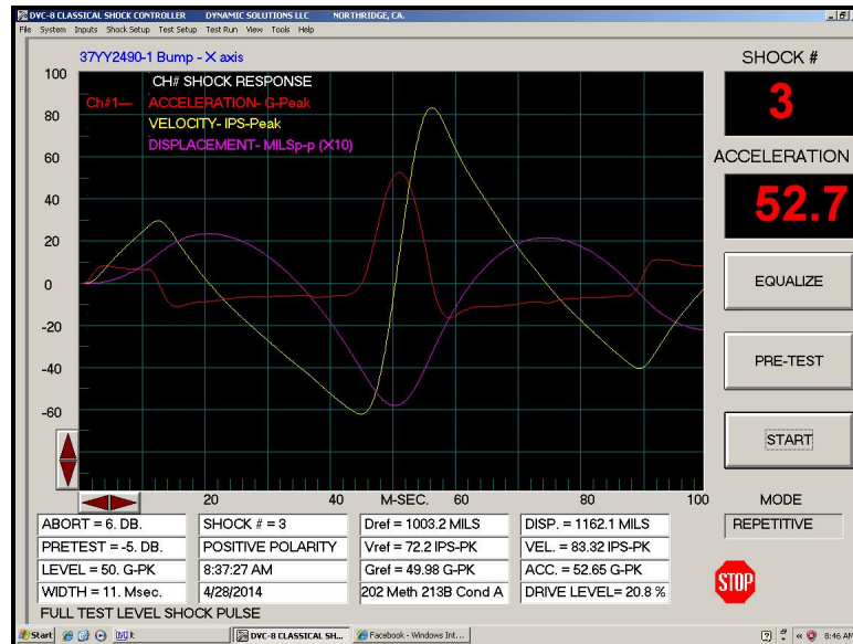
Figure 18 – Mechanical Shock Wave Form
