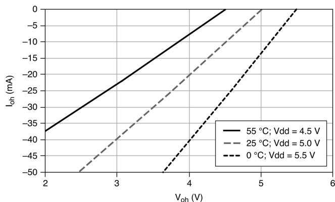
Figure 5. DIO (PFI <0..15>/P1/P2): I_{oh} versus V_{oh}
