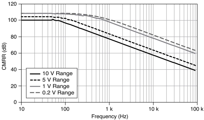
Figure 3. AI CMRR
