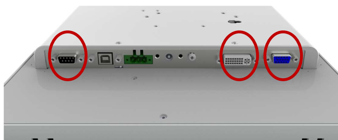
RS-232/DVI-D/VGA
