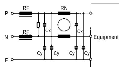
Figure 12. Two-stage powerline filter with differential- and common-mode suppression
