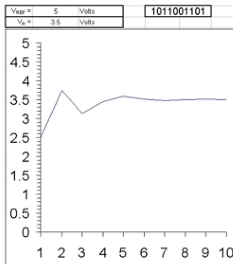
Figure 2. Successive Approximation Conversion by Russ Puskarcik—Own Work, CC BY 3.0, https://commons.wikimedia.org/w/index.php?curid=39713802
