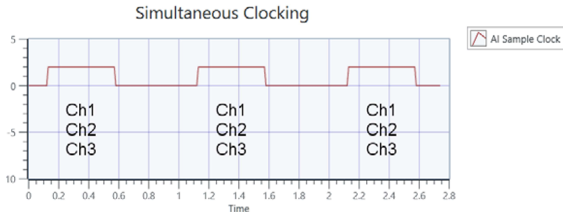
Figure 9. Each tick of the sample clock triggers acquisition on all active channels.
