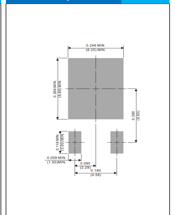
TO-252AA Pad Layout Unit: inch(mm)
