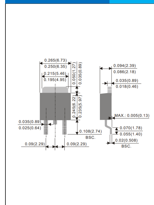
TO-252AA Dimension Unit: inch(mm)
