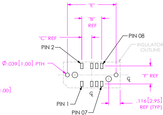
FIG. 2 -05 POSITION WITH -WT OPTION SHOWN (SAME AS FIG. 1, EXCEPT AS SHOWN)
