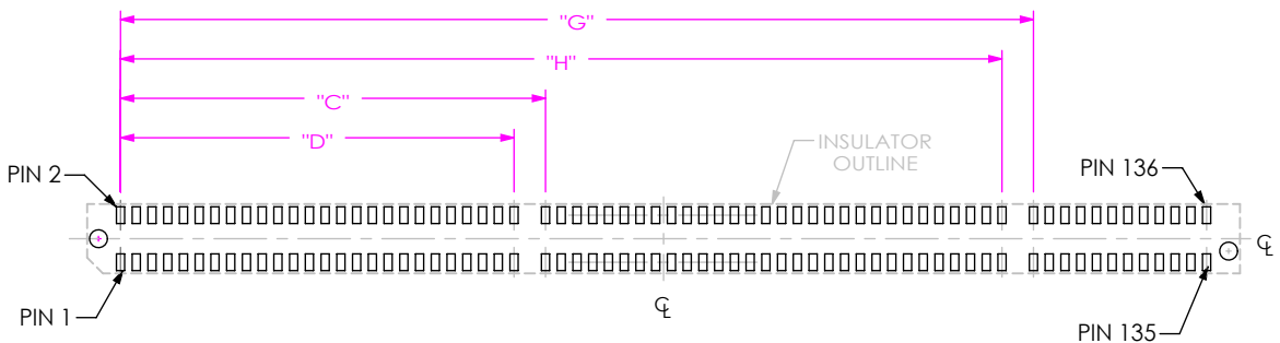
FIG. 4 -70 POSITION SHOWN (SAME AS FIG. 1, EXCEPT AS SHOWN) (NOT TOOLED)
