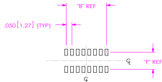
FIG. 3 -08 POSITION SHOWN (NON-POLARIZED) (SAME AS FIG. 1, EXCEPT AS SHOWN) (NOT TOOLED)
