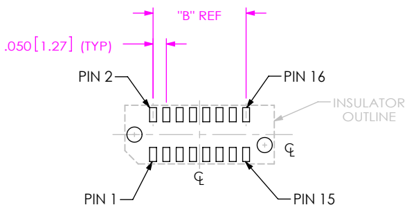
FIG. 3 -08 POSITION SHOWN (NON-POLARIZED) (SAME AS FIG. 1, EXCEPT AS SHOWN) (NOT TOOLED)
