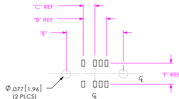
FIG. 2 -05 POSITION WITH -WT OPTION SHOWN (SAME AS FIG. 1, EXCEPT AS SHOWN)
