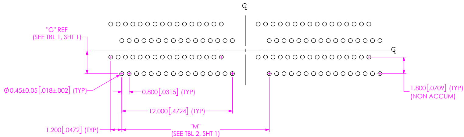
FIG 2 NVAF-DP-04-2-XX.X-X-X-K-XR STENCIL SHOWN
