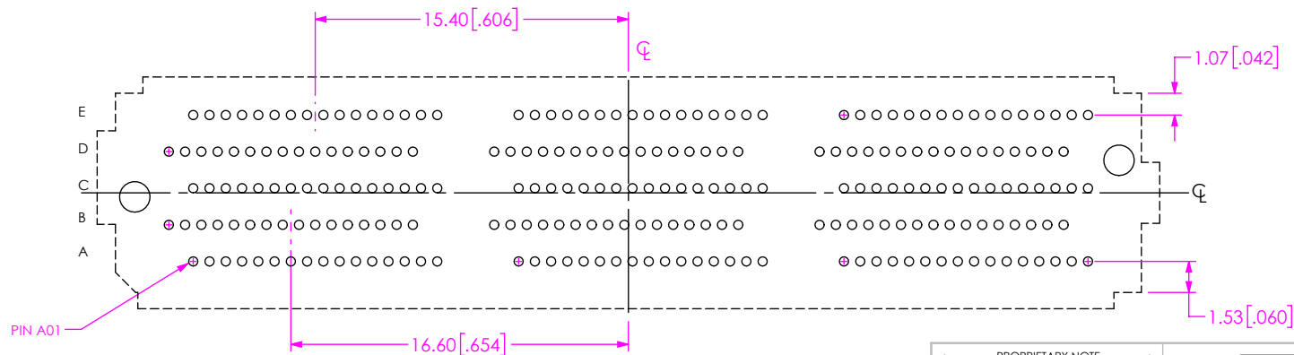
FIG 13 (NVAF-3 BANK SHOWN)
