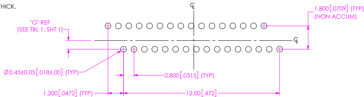
FIG 4 NVAF-DP-02-1-XX.X-X-X-K-XR STENCIL SHOWN
