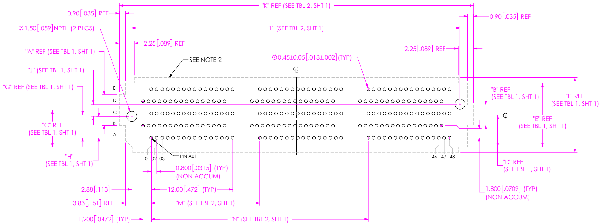
FIG 7 NVAF-DP-05-3-XX.X-X-X-K-XR FOOTPRINT SHOWN (SAME AS FIGURE 1, EXCEPT AS SHOWN)
