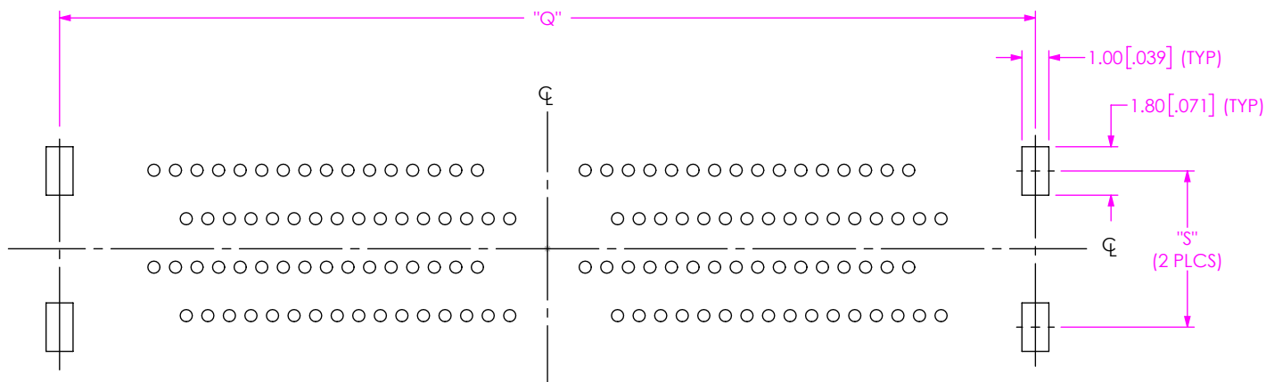
FIG 15 NVAF-DP-04-2-XX.X-X-X-WT-K-XR STENCIL SHOWN (SAME AS FIGURE 2, EXCEPT AS SHOWN)
