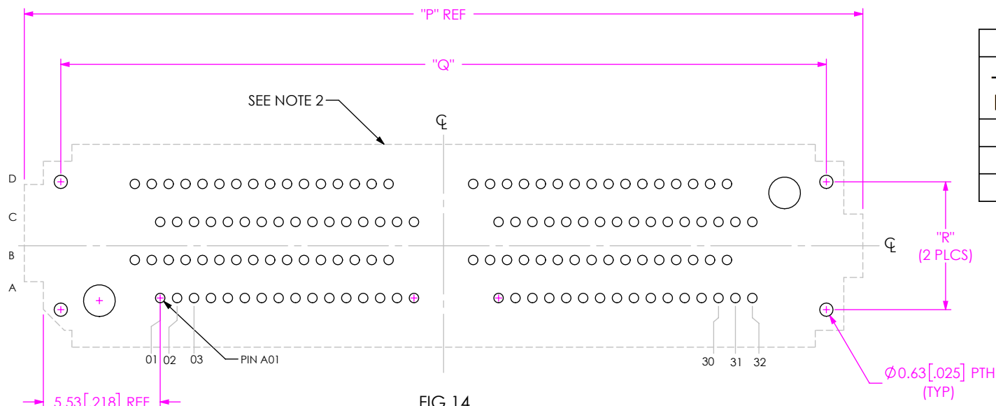
FIG 14 NVAF-DP-04-2-XX.X-X-X-WT-K-XR FOOTPRINT SHOWN (SAME AS FIGURE 1, EXCEPT AS SHOWN)
