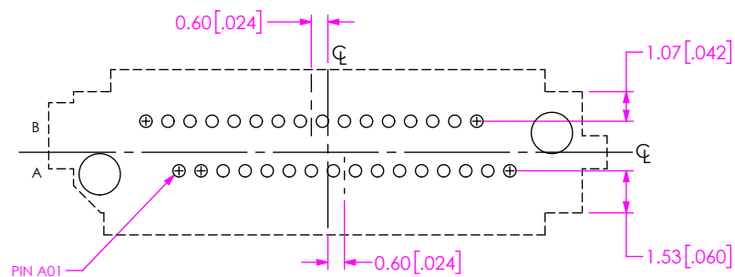
FIG 11 (NVAF-1 BANK SHOWN)
