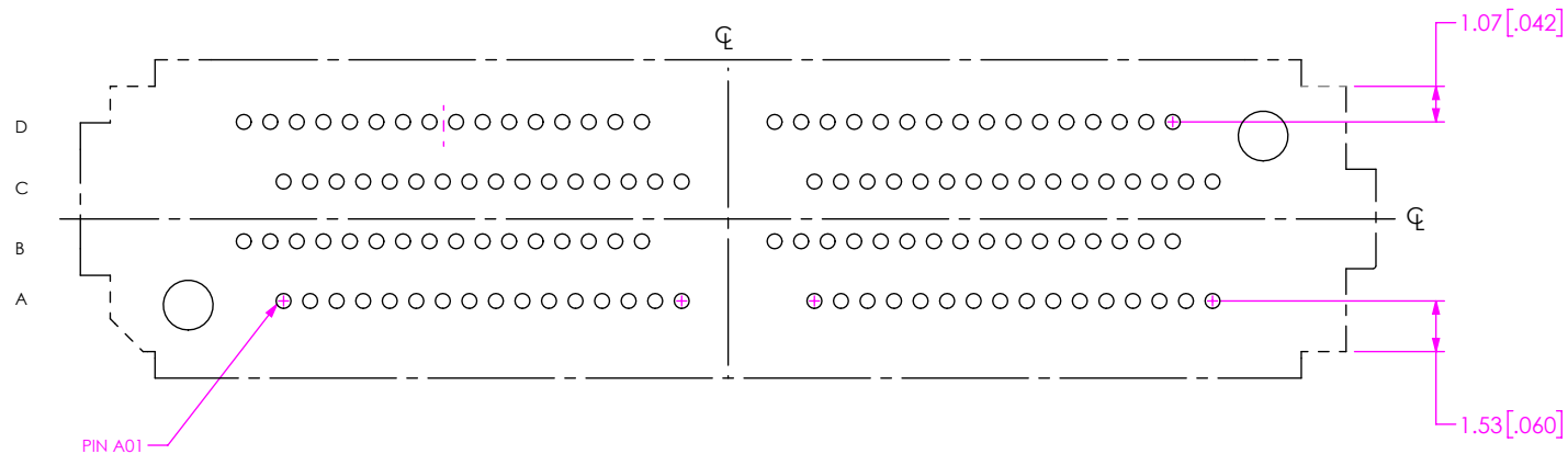
FIG 16 (NVAF-2 BANK WITH -WT OPTION SHOWN) (SAME AS FIGURES 11, 12 & 13)
