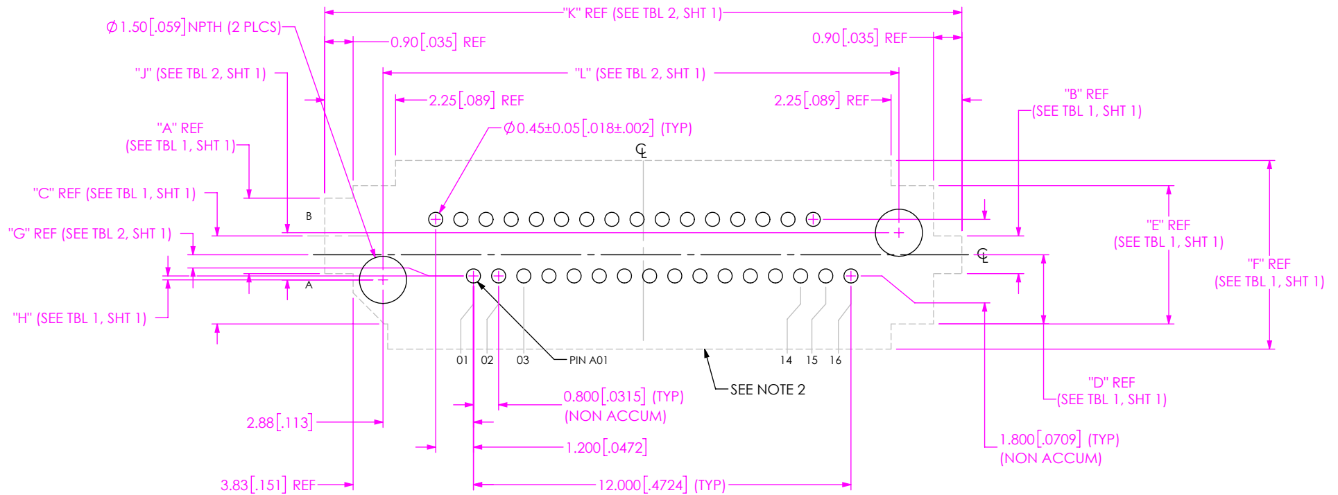
FIG 3 NVAF-DP-02-1-XX.X-X-X-K-XR FOOTPRINT SHOWN (SAME AS FIGURE 1, EXCEPT AS SHOWN)
