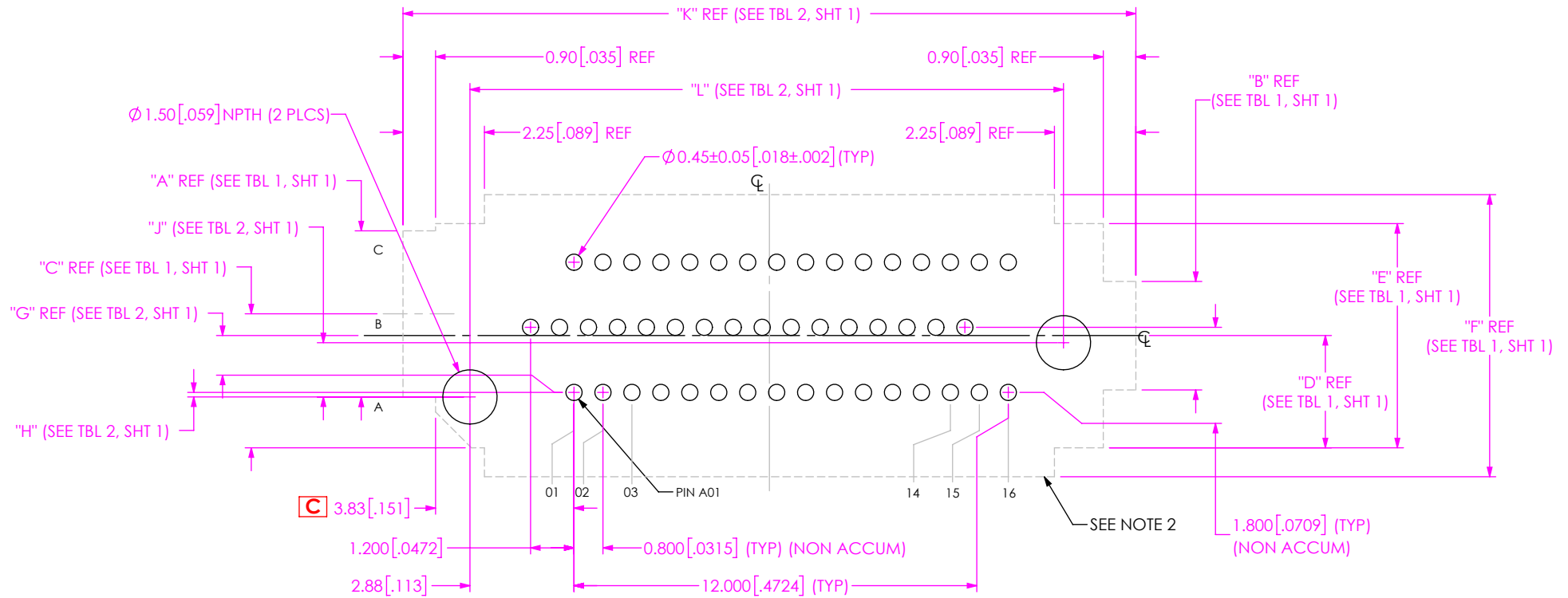
FIG 5 NVAF-DP-03-1-XX.X-X-X-K-XR FOOTPRINT SHOWN (SAME AS FIGURE 1, EXCEPT AS SHOWN)
