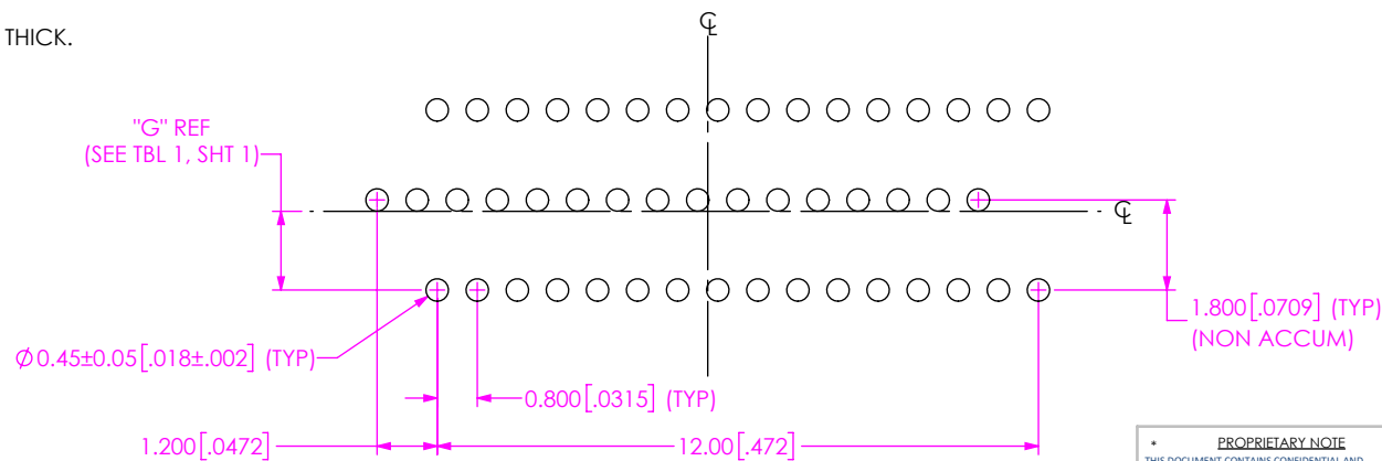
FIG 6 NVAF-DP-03-1-XX.X-X-X-K-XR STENCIL SHOWN
