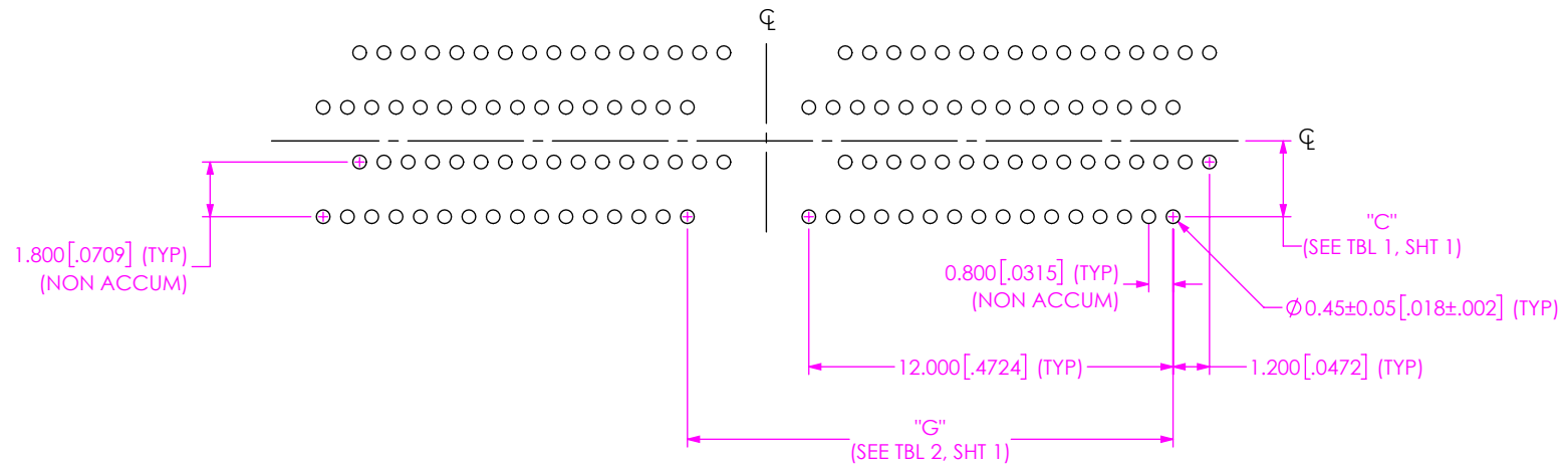
FIG 2 NVAM-DP-04-2-XX.X-X-X-XX-K-XR STENCIL SHOWN
