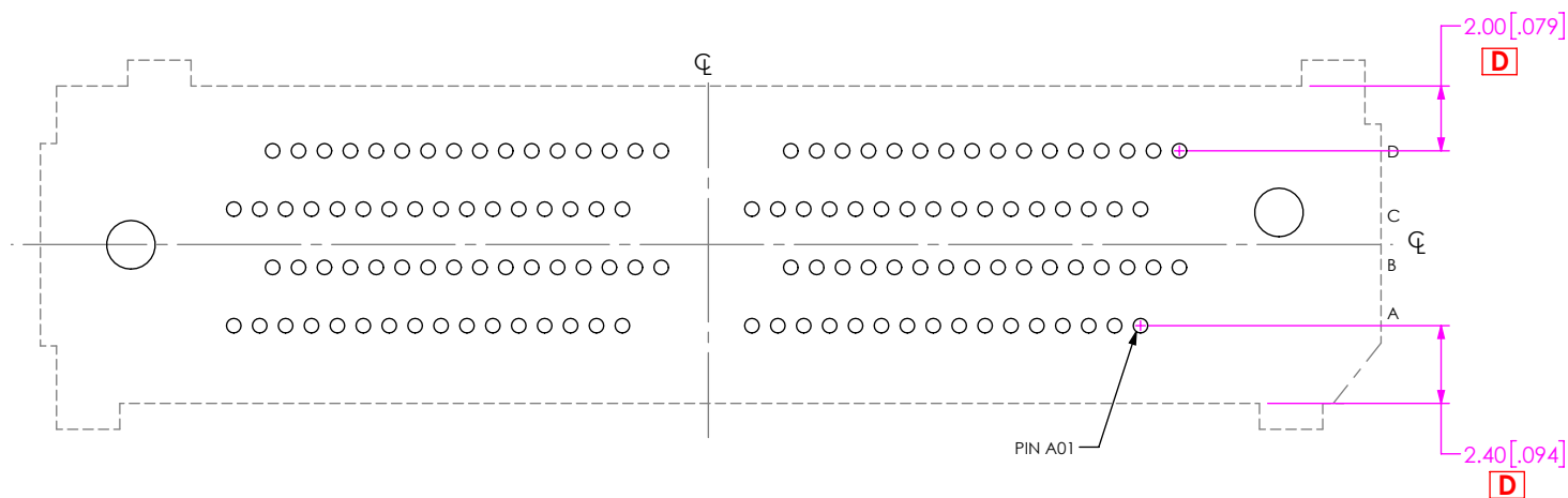
FIG 16 (NVAM-2 BANK WITH -WT OPTION SHOWN) (SAME AS FIG 11, 12 & 13)
