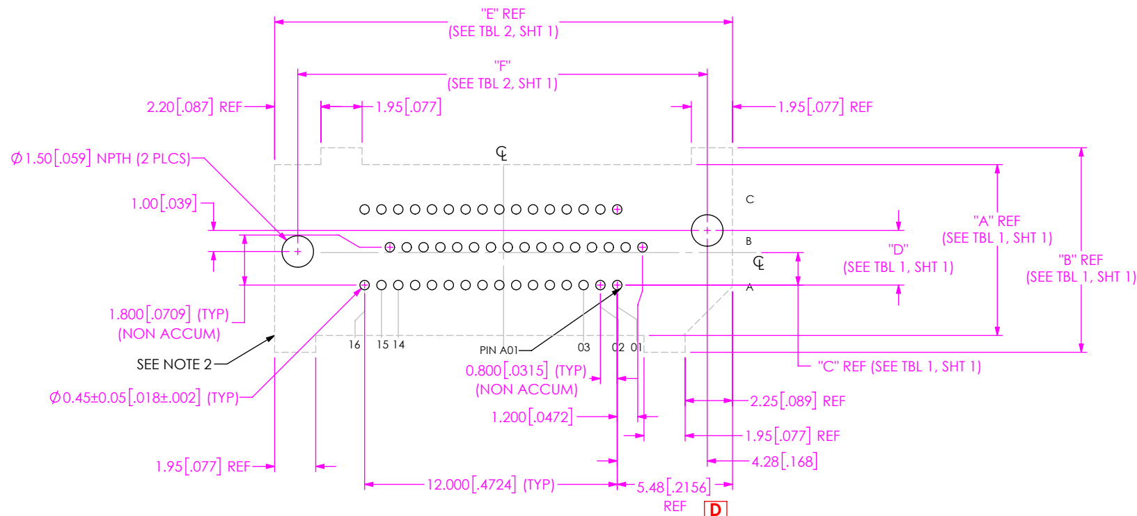
FIG 5 NVAM-DP-03-1-XX.X-X-X-XX-K-XR FOOTPRINT SHOWN (SAME AS FIG 1, EXCEPT AS SHOWN)
