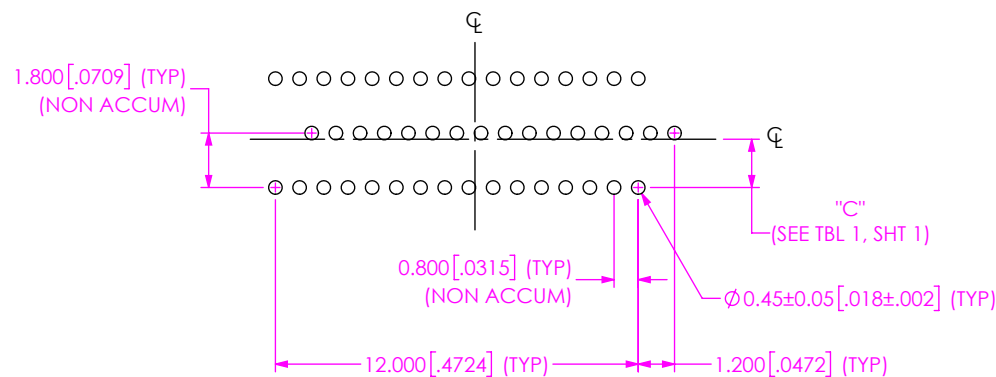
FIG 6 NVAM-DP-03-1-XX.X-X-X-XX-K-XR STENCIL SHOWN
