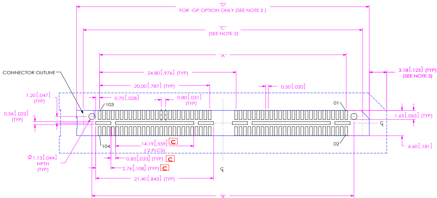
FIG 1 [C] QRF8-052-XX.X-X-D-A SHOWN
