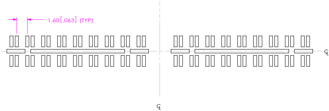
FIG 4 C QRF8-036-XX.X-X-DP-A SHOWN (DIFFERENT AS SHOWN, OTHERWISE SAME AS FIG 3)
