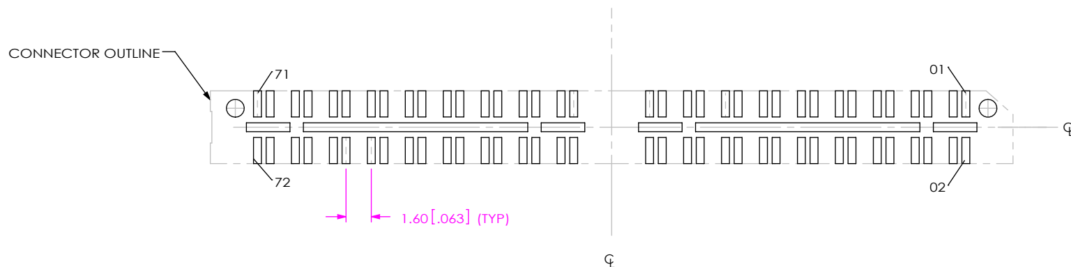
FIG 3 C QRF8-036-XX.X-X-DP-A SHOWN (DIFFERENT AS SHOWN, OTHERWISE SAME AS FIG 1)
