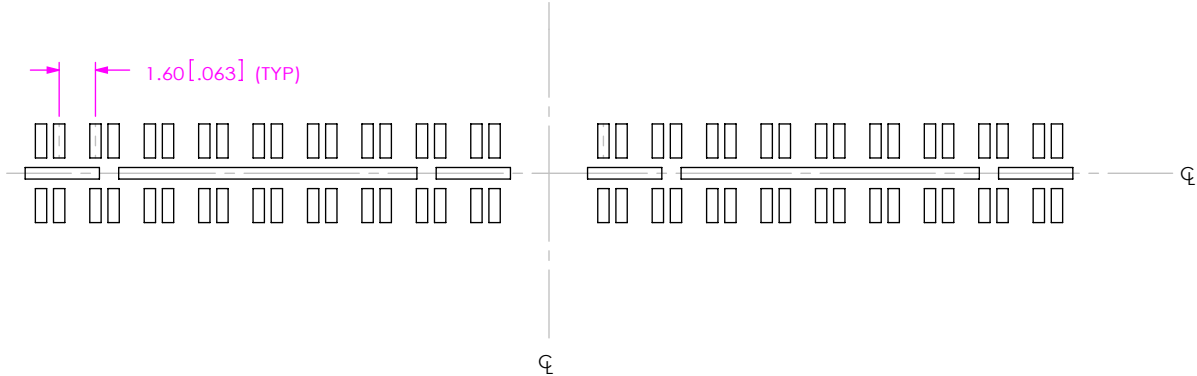
C FIG 4 QRM8-036-XX.X-X-DP-A SHOWN (DIFFERENT AS SHOWN, OTHERWISE SAME AS FIG 3)
