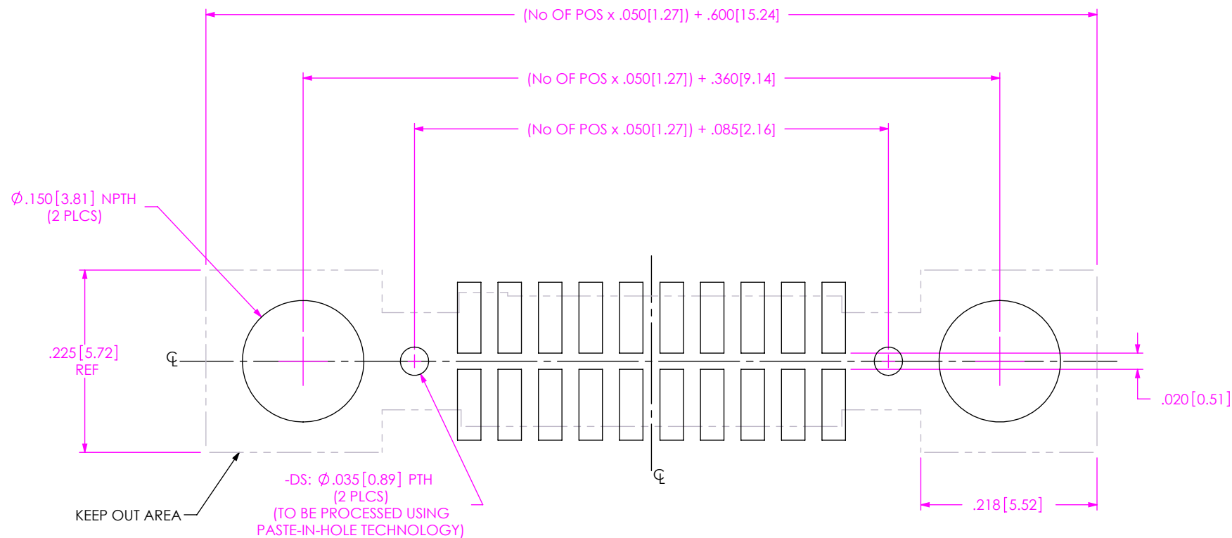
FIG 2 -DS OPTION SAME AS FIG 1 EXCEPT AS SHOWN
