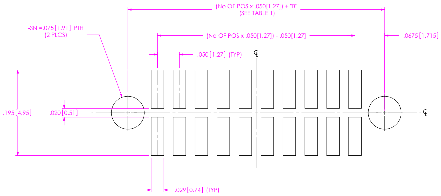
FIG 3 SAME AS FIG 1 EXCEPT AS SHOWN
