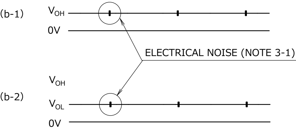
(b) IN CASE OF STEADY LOCKED ROTOR
