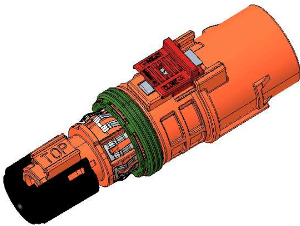
Diecast with round corner
