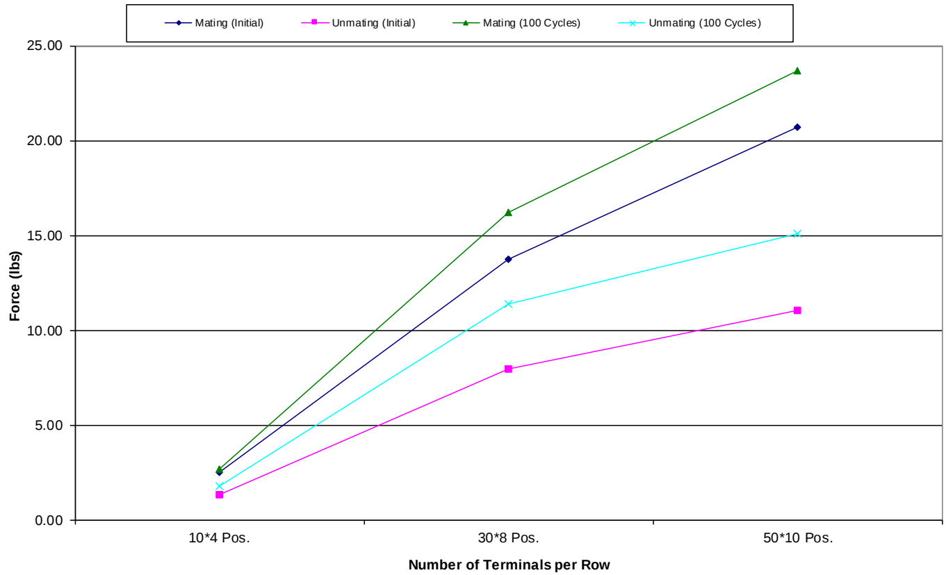
Mating/Unmating Data for 10*4, 30*8 and 50*10 Position SEAF/SEAM
