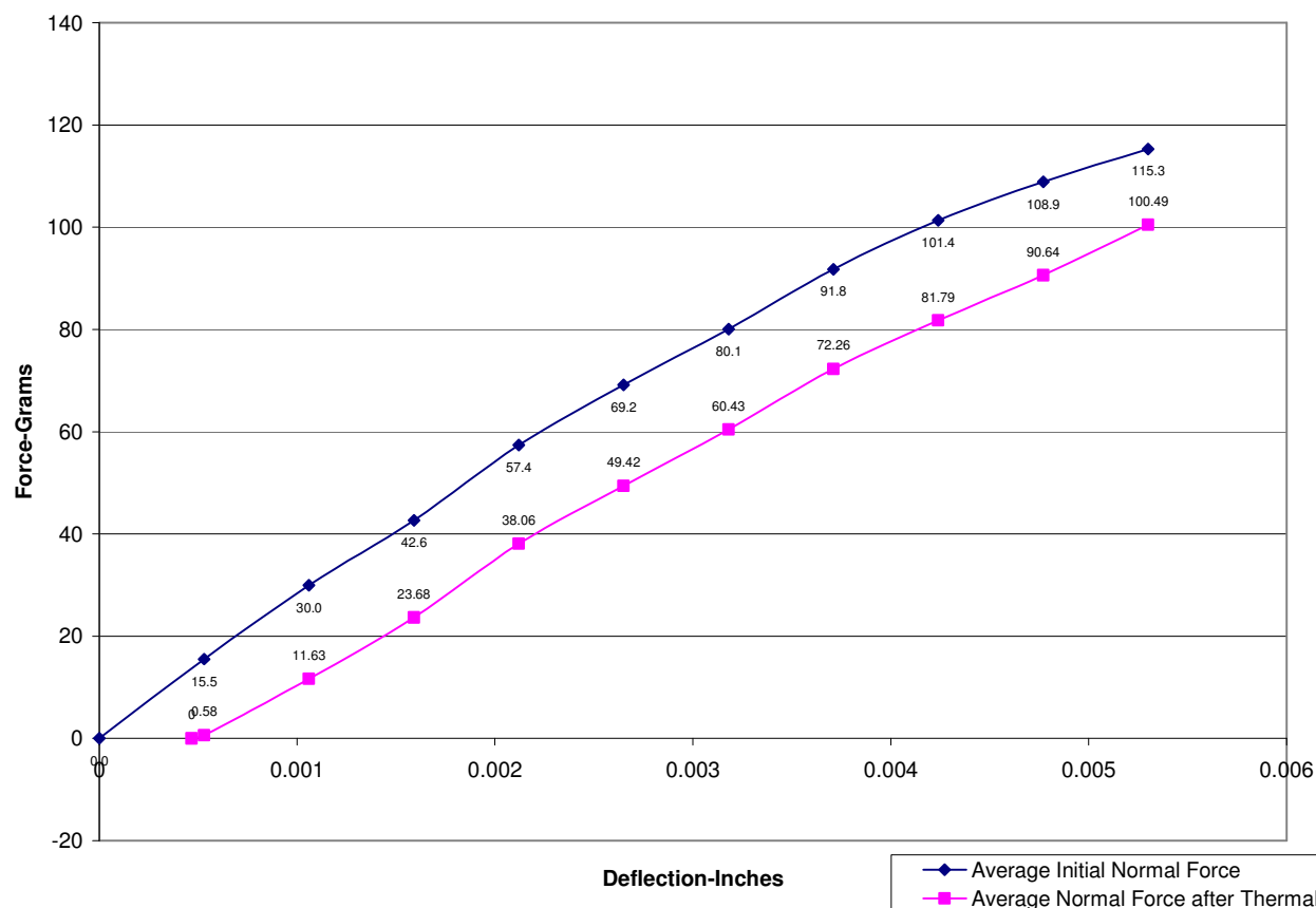
Normal Force - Average Initial vs Average Thermal
