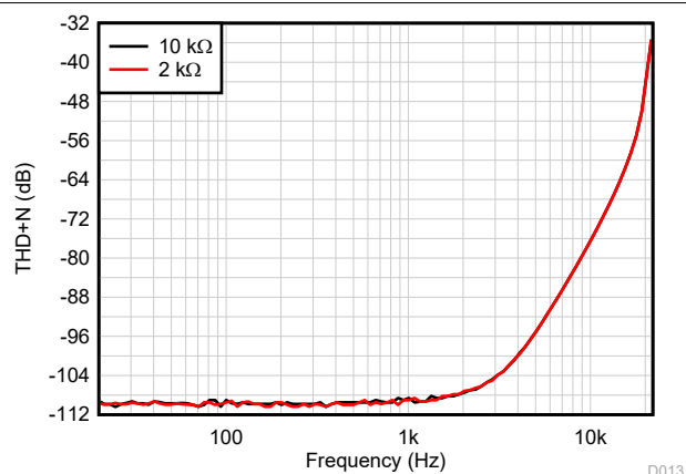
G = 1 , f = 1\text{ kHz} , BW = 80\text{ kHz} , V_{OUT} = 10\text{ V}_{PP} , R_L connected to V_- Figure 7-18. THD+N Ratio vs Frequency, G = 1
